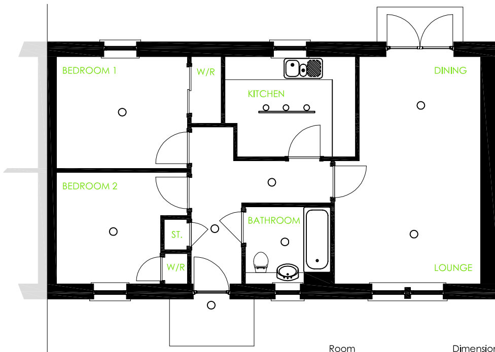
FLOOR PLAN
